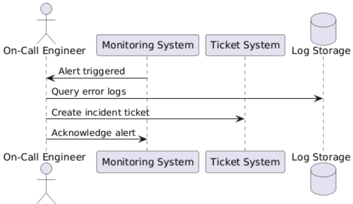
Diagram 1: Sequence diagram of incident response
