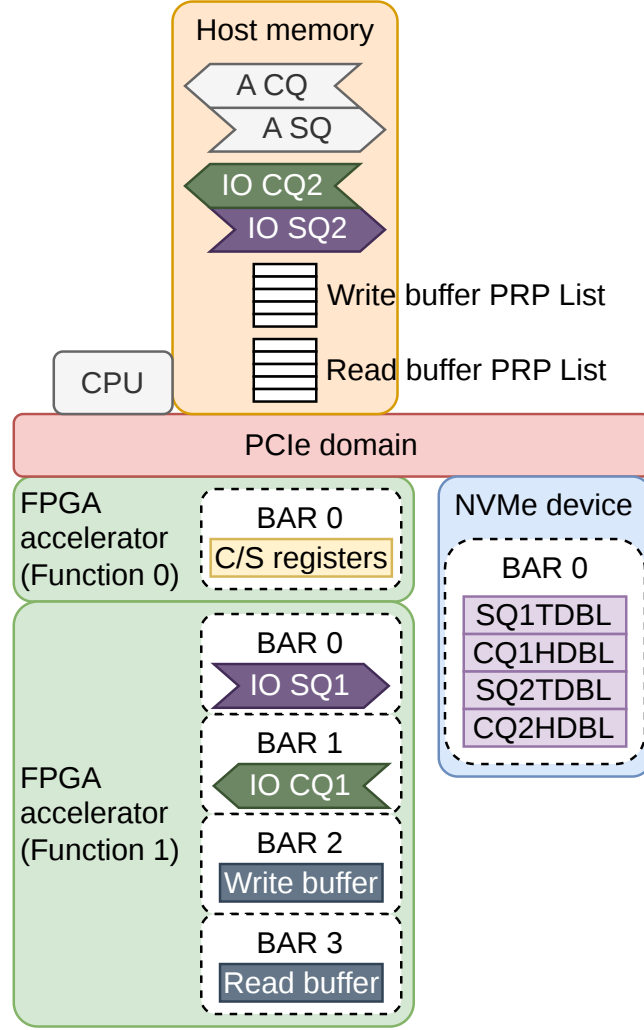
Fig. 4.4: Overview of allocated memory resources as initialized by the SPDK application.
