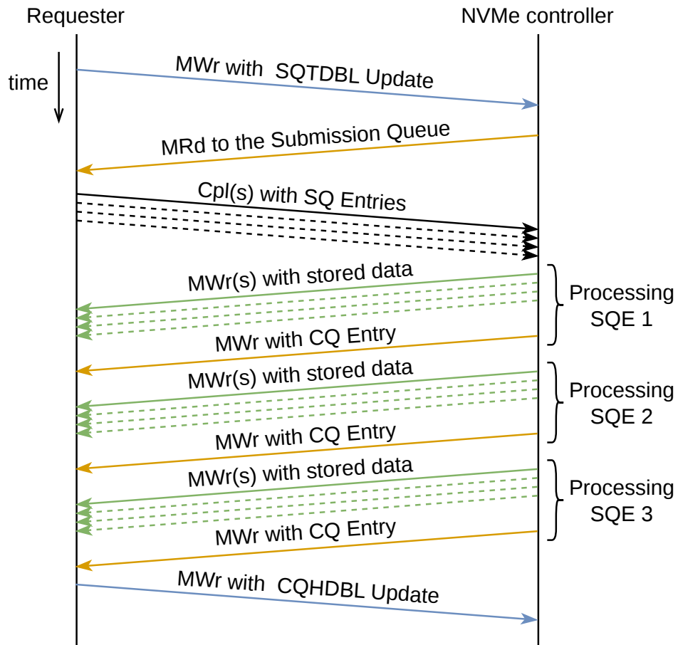
Fig. 4.4: Read command submission. The indexing of SQEs is completely arbitrary since there is no ordering of commands on the NVMe controller's side if multiple commands are fetched.
