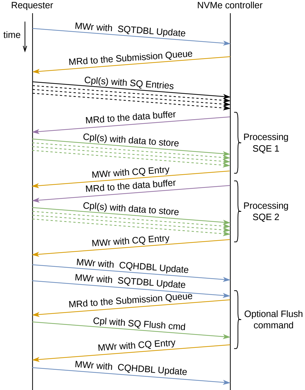
Fig. 4.5: Write command submission. The indexing of SQEs is completely arbitrary since there is no ordering of commands on the NVMe controller's side if multiple commands are fetched.
