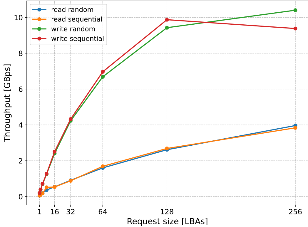
Fig. 6.2: Measured throughput for different numbers of copied LBAs and access patterns. The write operation exceeds the theoretical maximum, which is probably caused by fluctuating data rate on the PCIe chain.
