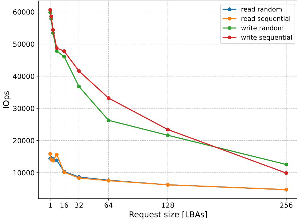
Fig. 6.1: Measured IOps for different numbers of copied LBAs and access patterns
