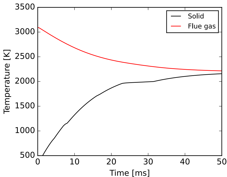
Figure 7.1: Verification of single particle heating thermal history.
