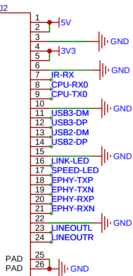
FPC-0.5MM-24P
