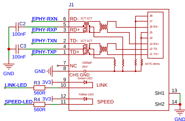
Ethernet (10/100M)
