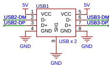
USB X 2
