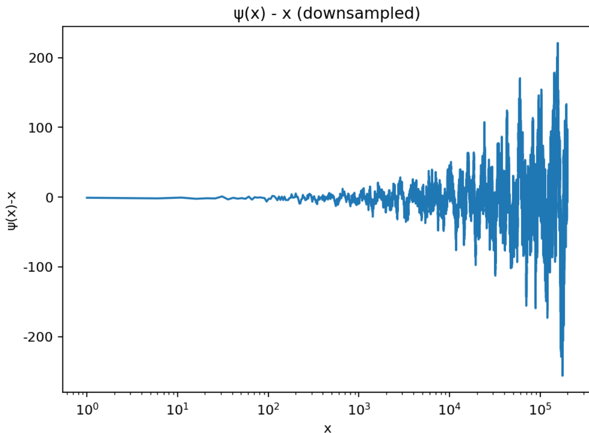
Fig. 22: E103 — Chebyshev (x): prime powers drive jumps
