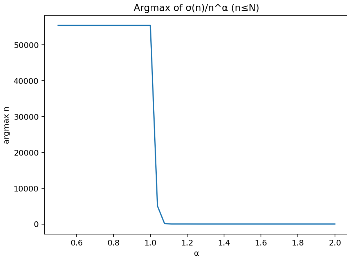
Fig. 17: E098 — Maximizers of (n)/n^\alpha across
