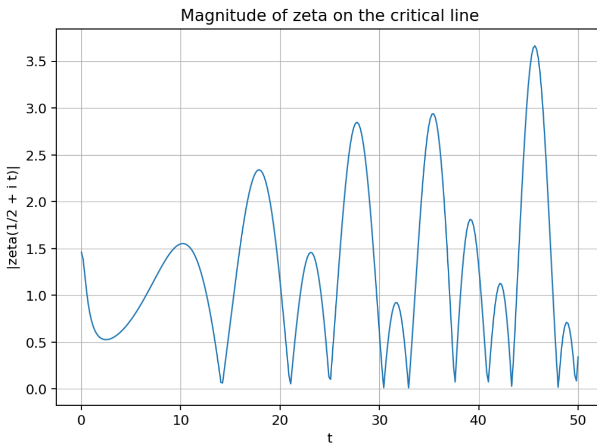
Fig. 3: E084 — |\zeta(1/2+it)| growth snapshots
