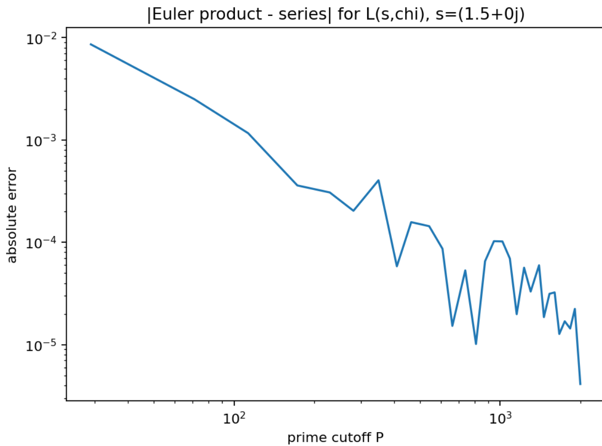
Fig. 31: E111 — Euler product vs. Dirichlet series for L(s, )
