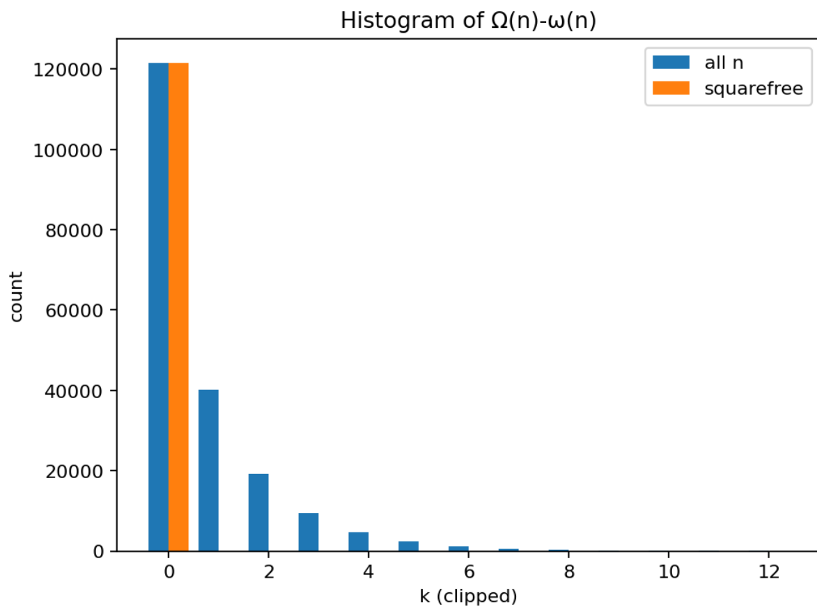
Fig. 14: E095 — Squarefree filter: (n)=\Omega(n) when (n)\neq 0
