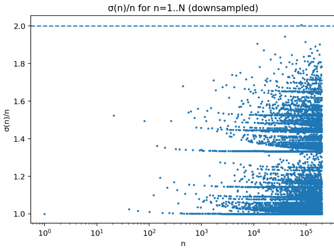
Fig. 16: E097 — (n)/n landscape: deficient, perfect, abundant
