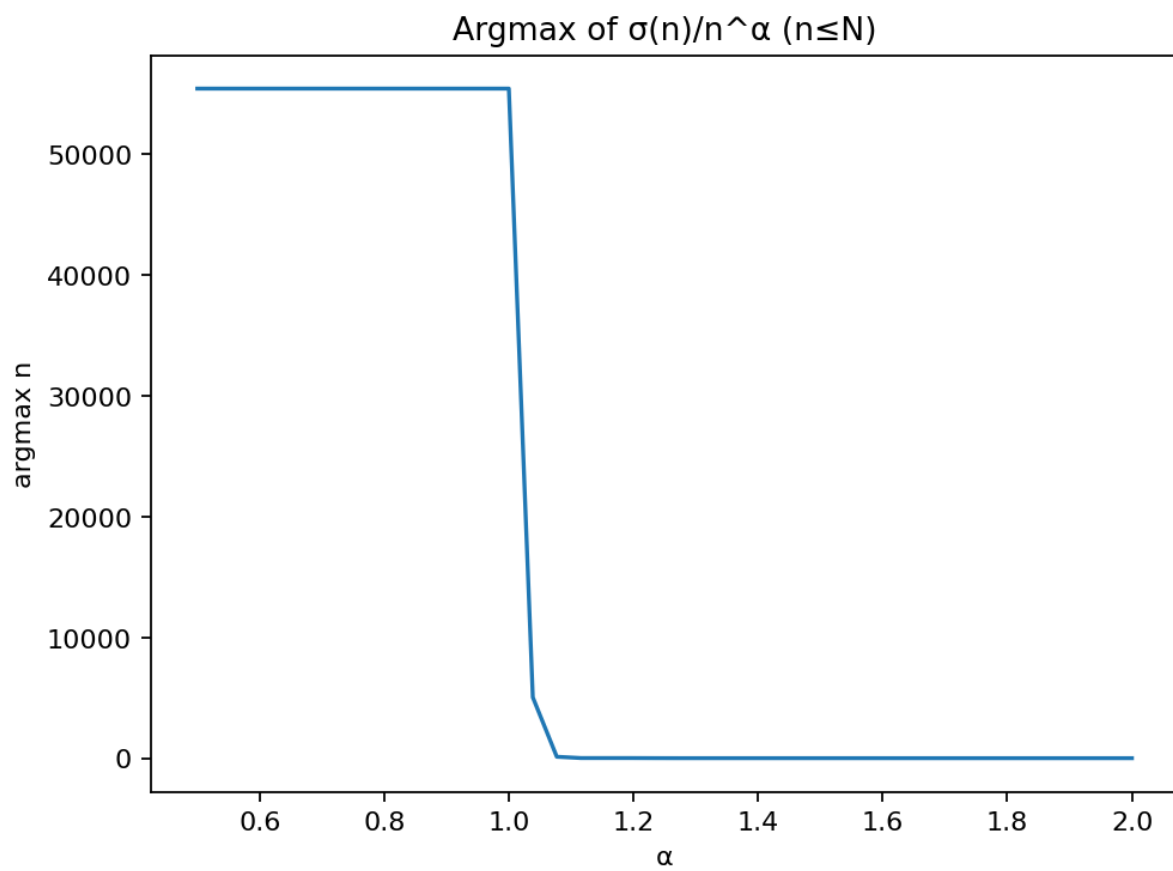
Fig. 17: E098 — Maximizers of \sigma(n)/n^\alpha across \alpha
