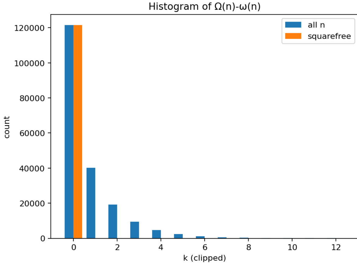
Fig. 14: E095 — Squarefree filter: (n)=\Omega(n) when (n) \leq 0
