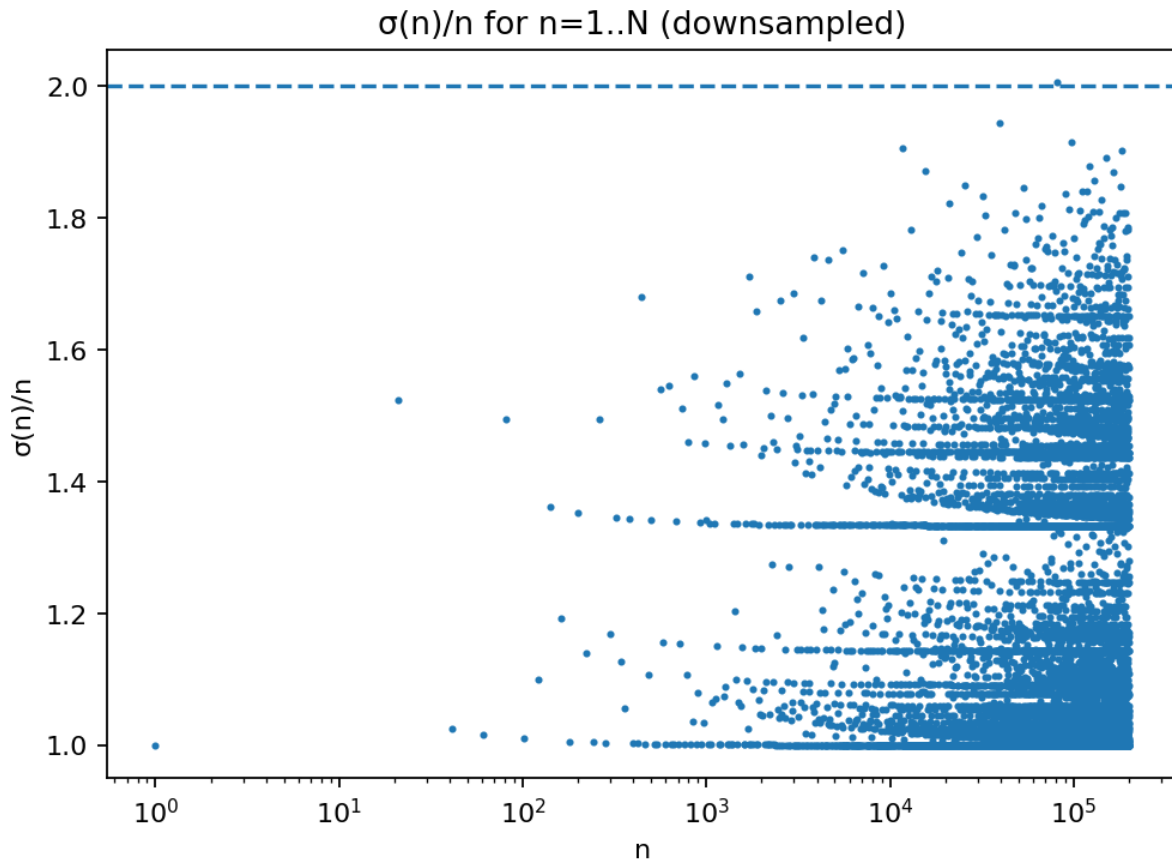
Fig. 16: E097 — (n)/n landscape: deficient, perfect, abundant
