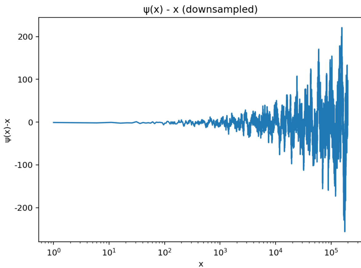
Fig. 22: E103 — Chebyshev \psi(x) : prime powers drive jumps
