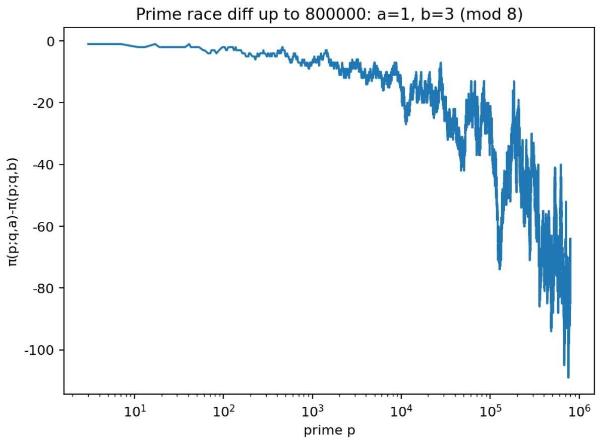
Fig. 32: E112 — Prime race: (x; q, a) - (x; q, b)
