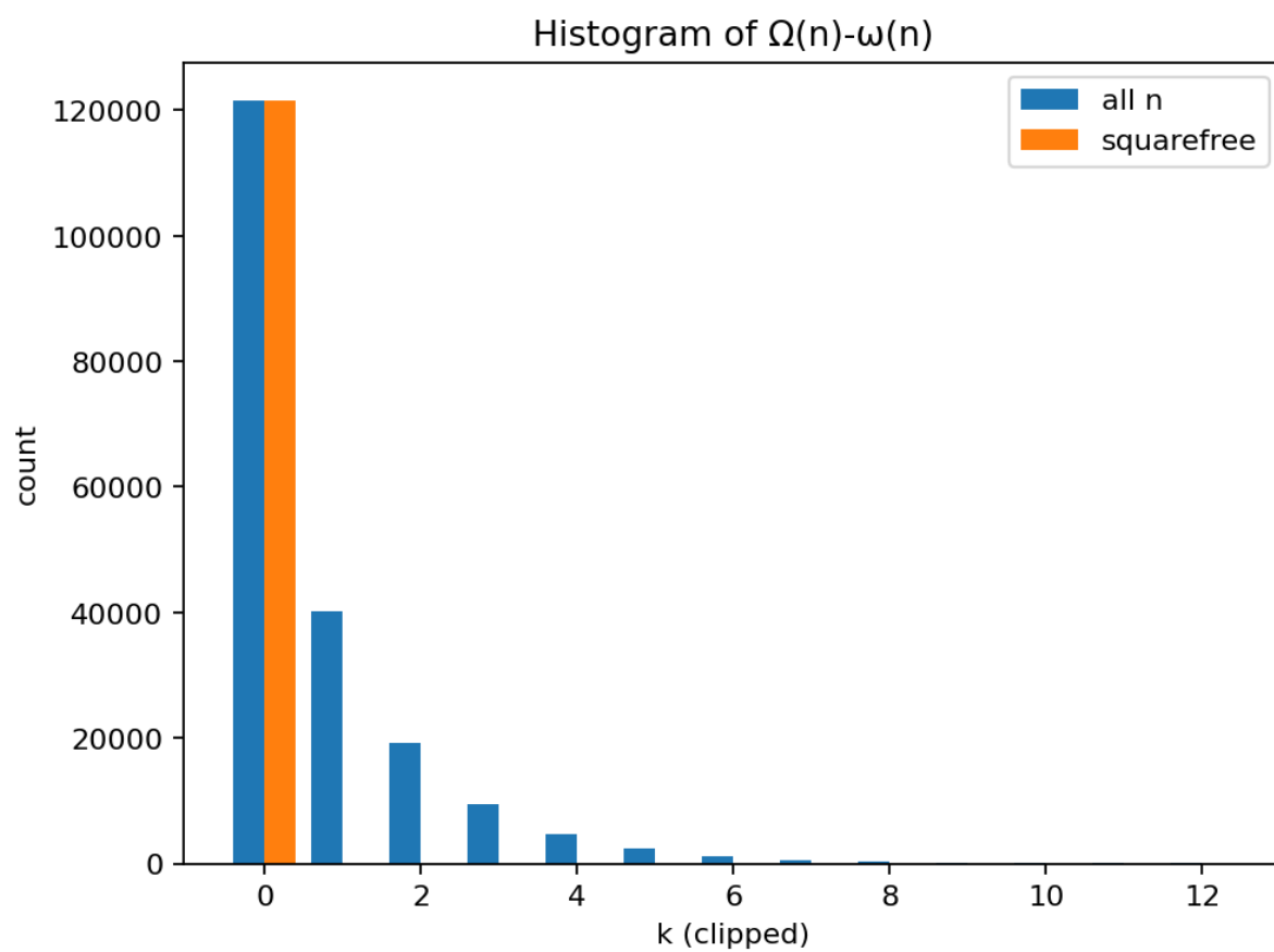
Fig. 14: E095 — Squarefree filter: \Omega(n)=\omega(n) when \Omega(n)=0
