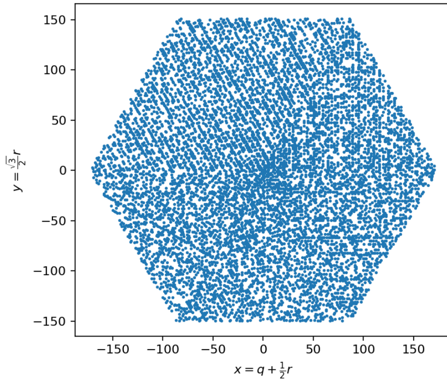
Hexagonal number spiral (primes, n \leq 90,601 , size=301)
