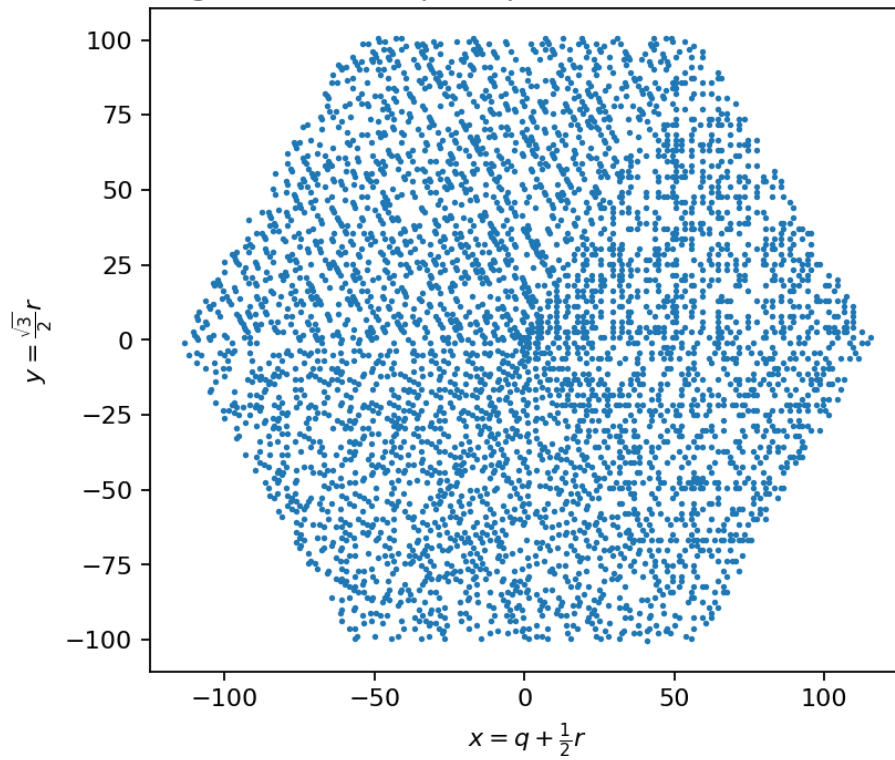
Hexagonal number spiral (primes, n \leq 40,401 , size=201)
