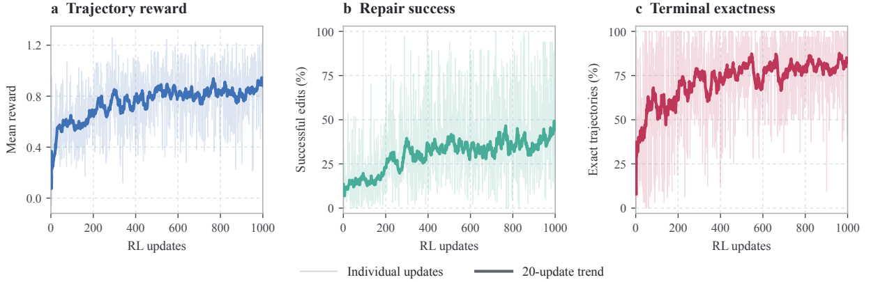
Figure 8 Learning dynamics of the 1,000-update RL run. (a) Mean trajectory reward. (b) Successful repairs per edit from an incorrect state. (c) Fraction of trajectories reaching terminal exactness under the training verifier. Faint lines are individual updates; solid lines are trailing 20-update trends, with rates pooling numerators and denominators over the window.
