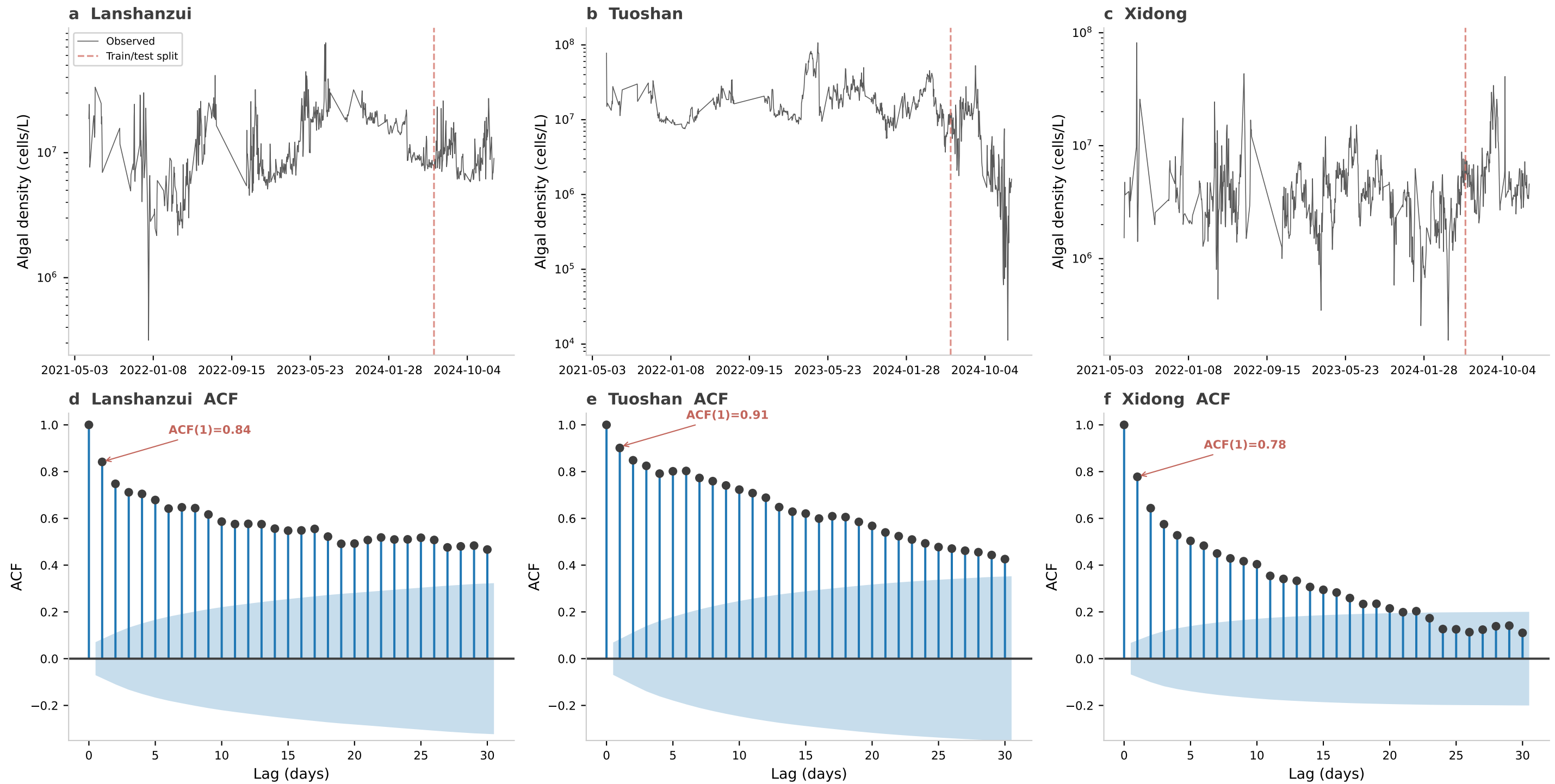
Figure 1. Time series and autocorrelation structure of log-transformed algal density
