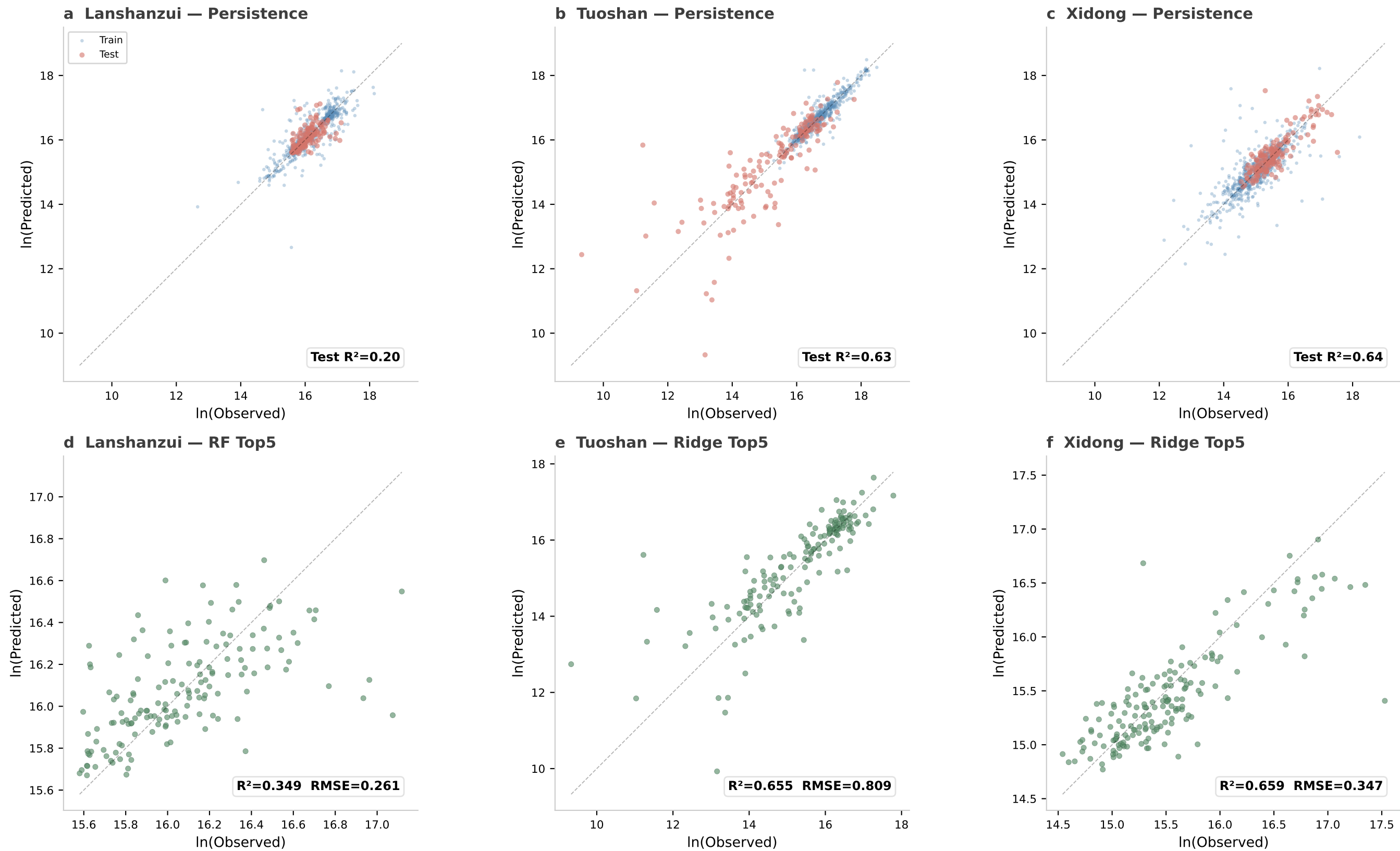
Figure 2. Observed vs. predicted values on the test set
