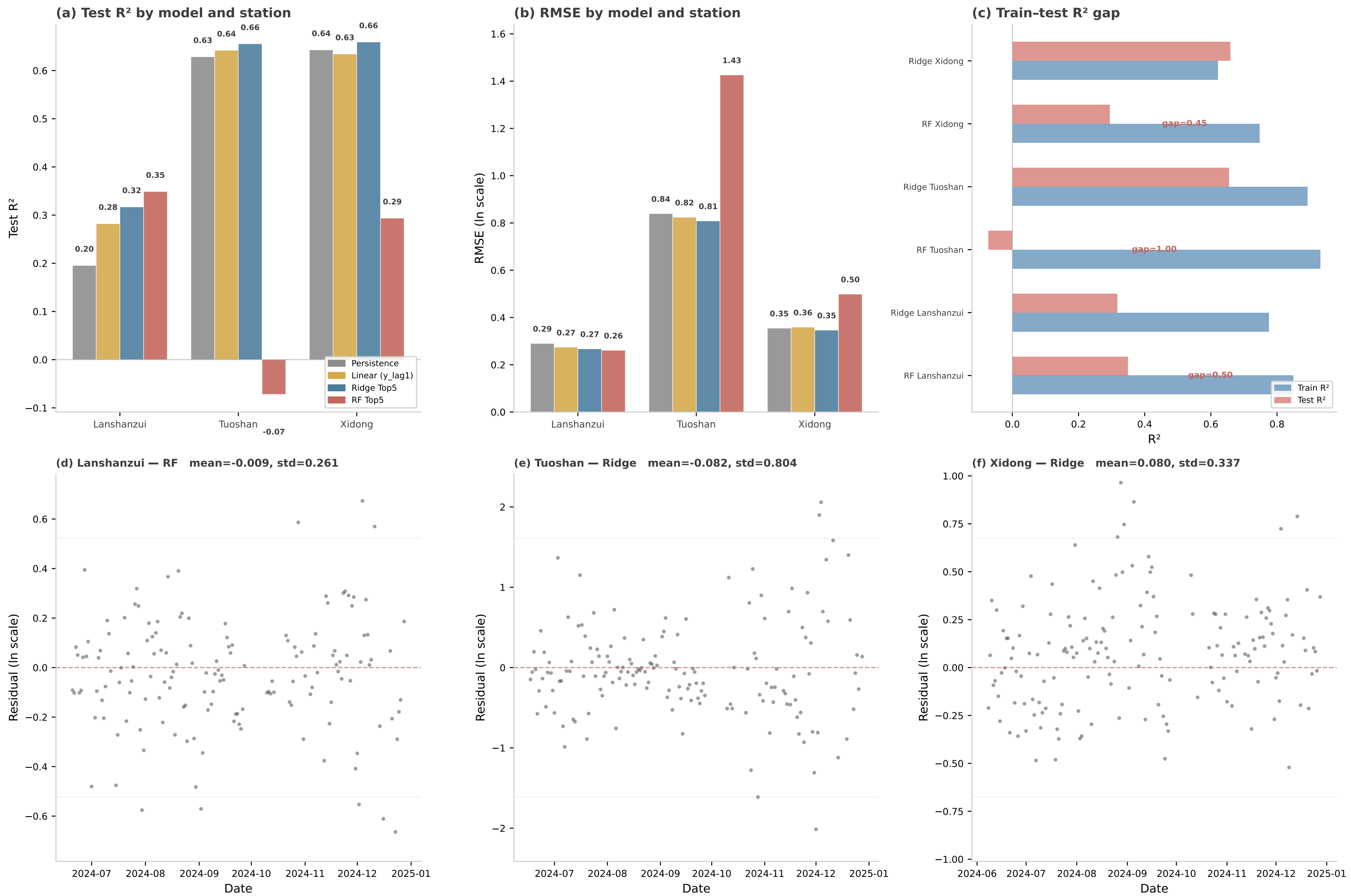
Figure 4. Model comparison and residual diagnostics
