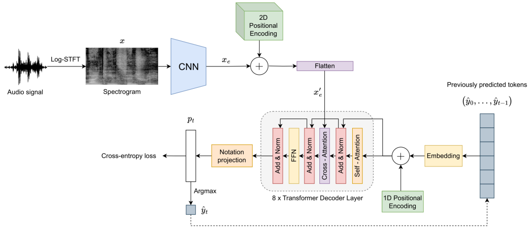
Fig. 1. Graphical scheme of the encoder-decoder proposal. The encoder is implemented as a CNN, whose output is added to a two-dimensional positional encoding before feeding the decoder, implemented as an auto-regressive Transformer.
