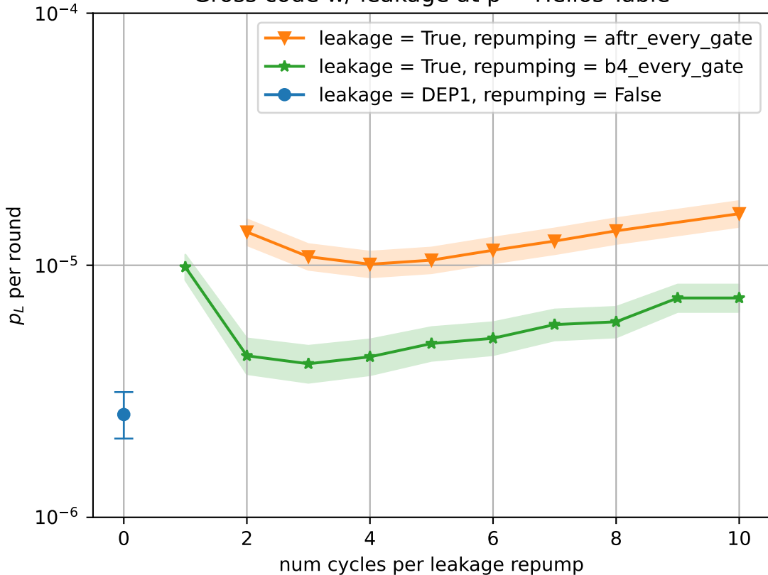
Gross code w/ leakage at p = Helios Table
