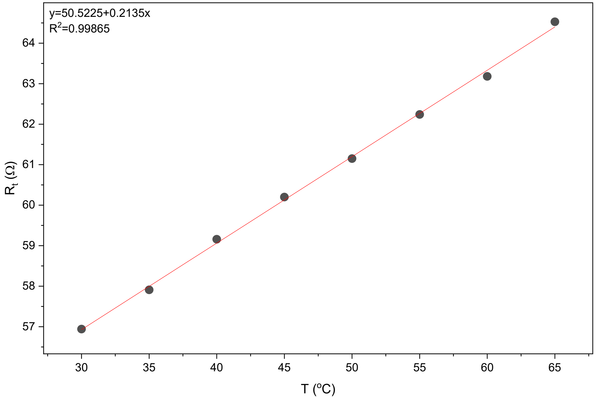
Linear Fit: R_t ( \Omega ) vs T ( ^{\circ}\text{C} )
