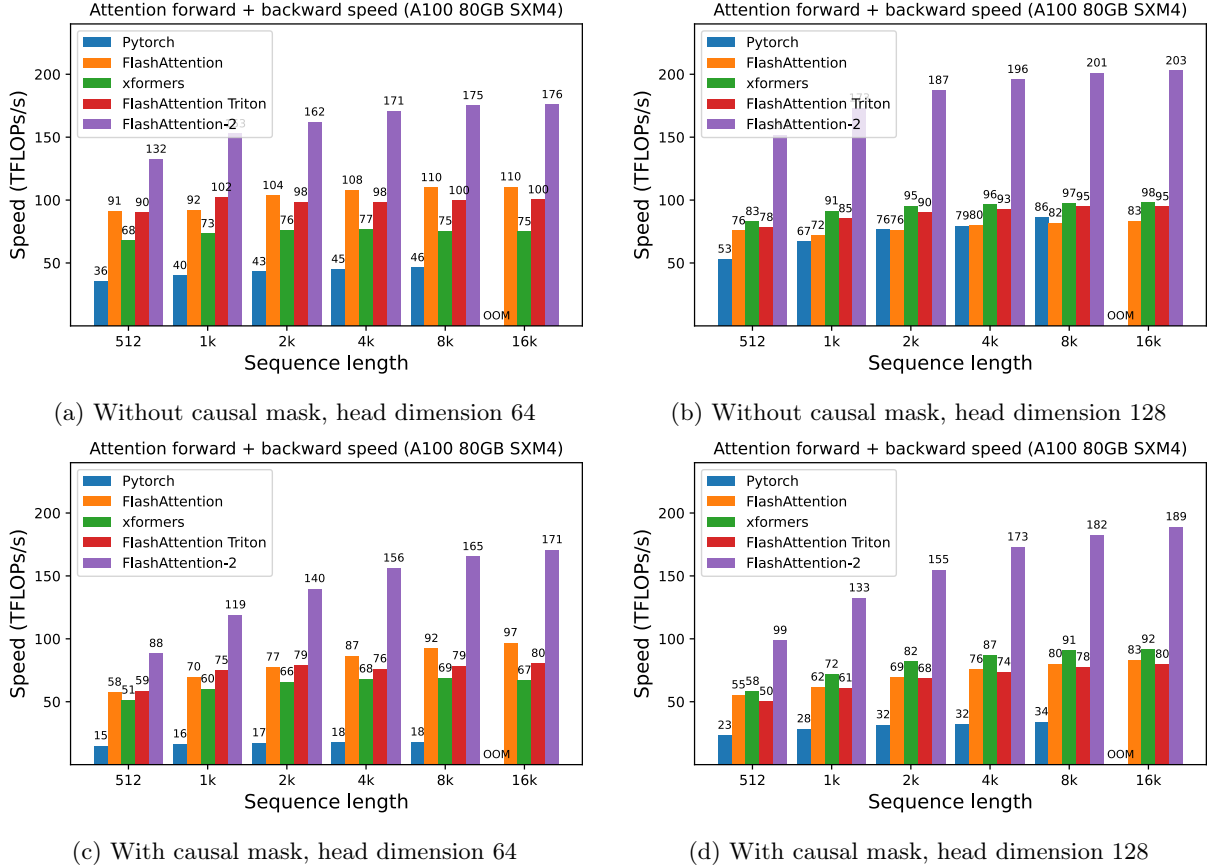
Figure 4: Attention forward + backward speed on 100 GPU
