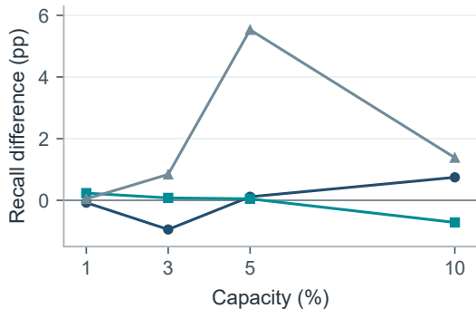
(a) IEEE-CIS: M2 – M0
