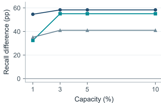
(b) PaySim: PTHW – P0
