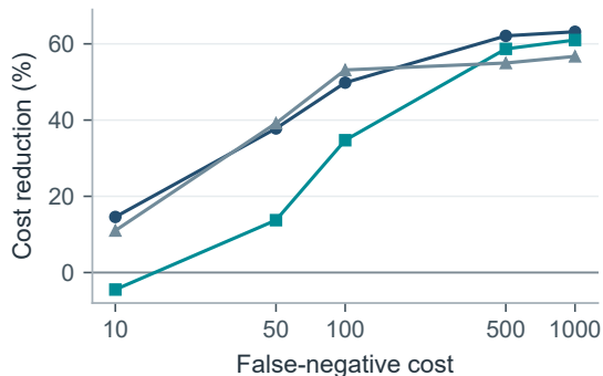
(c) PaySim: q = 3%
