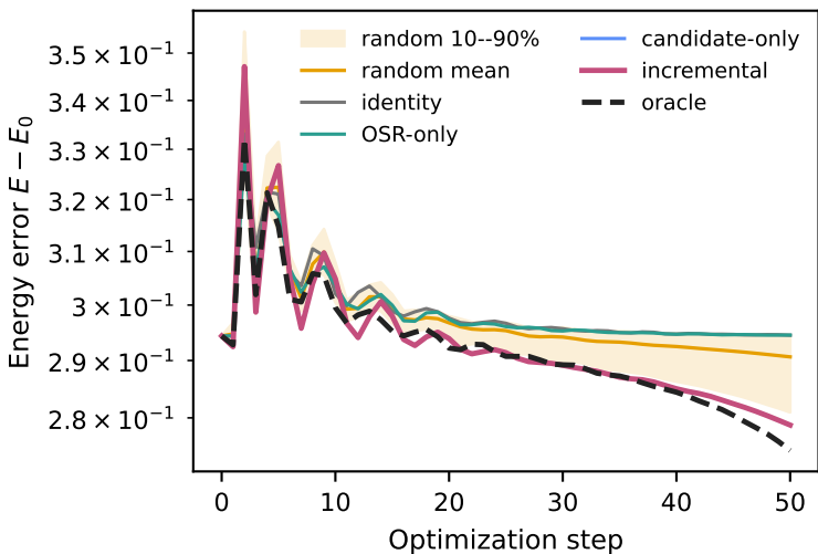
(a) Same-point TFIM intervention n=8, t=2
