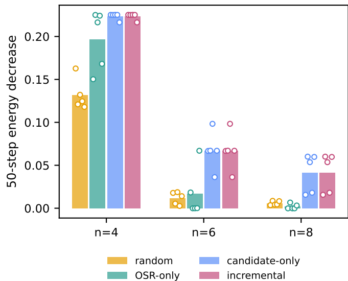
(c) Selection gains after retraining
