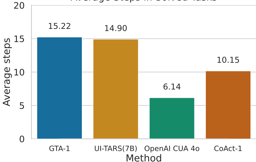
Average Steps in Solved Tasks
