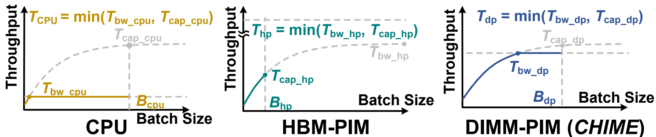
(c) Case studies of Liebig's Law
