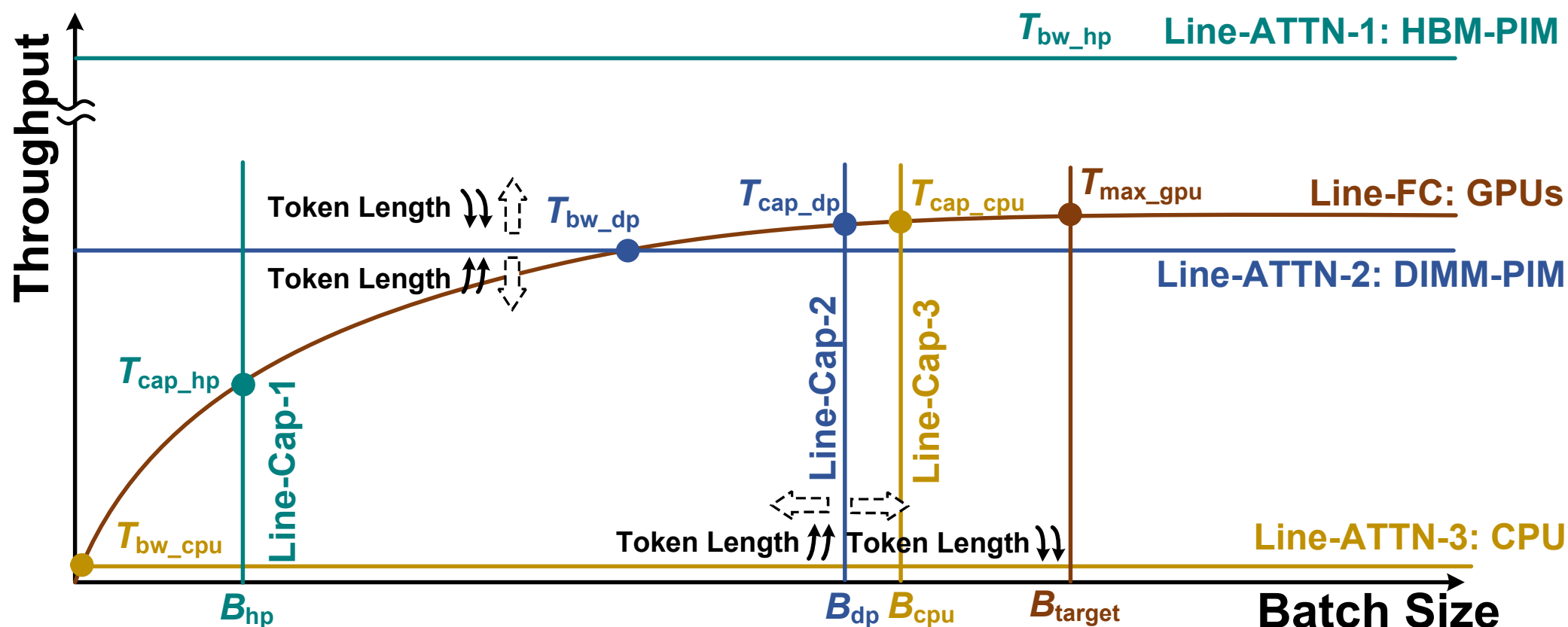
(b) Throughputs modeling of various AFD systems with DRM
