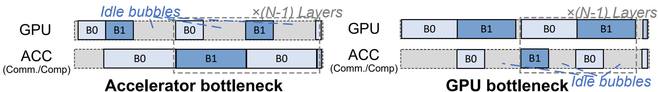
(a) Bottlenecks on two devices with sub-batch scheduling
