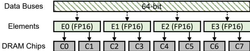
(a) DIMM-based transfer layout on 64-bit data buses
