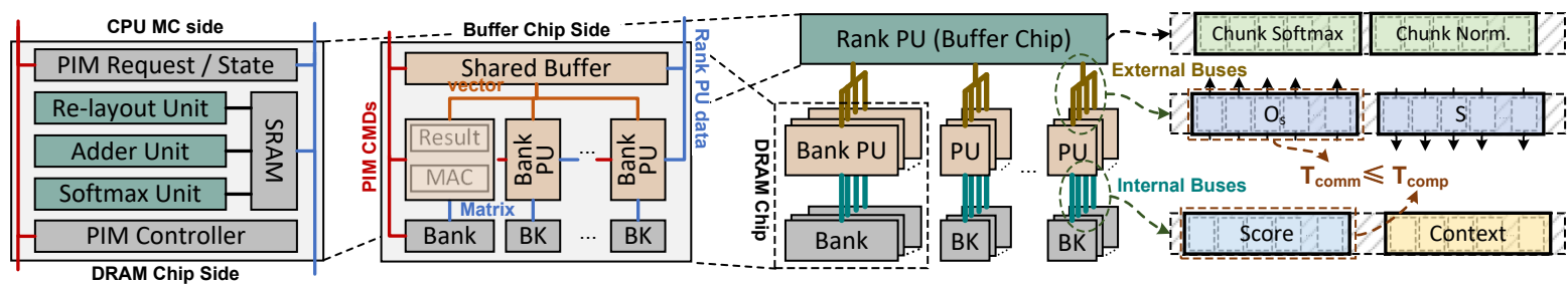
(a) CHIME-PIM rank PU and bank PU design
