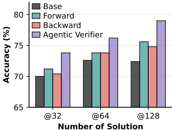
MATH500
