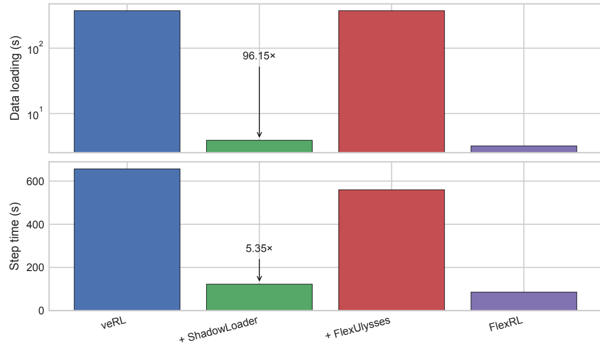
ShadowLoader Motivation (128×H800 GRPO workload)
