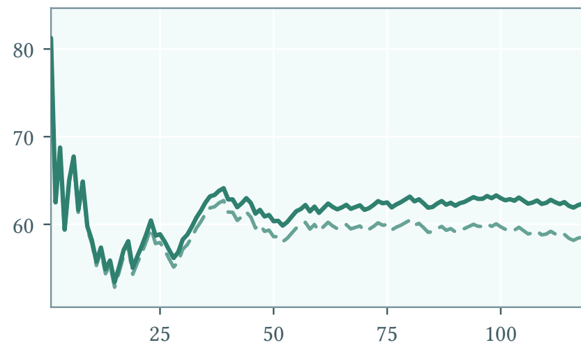
TravelPlanning
