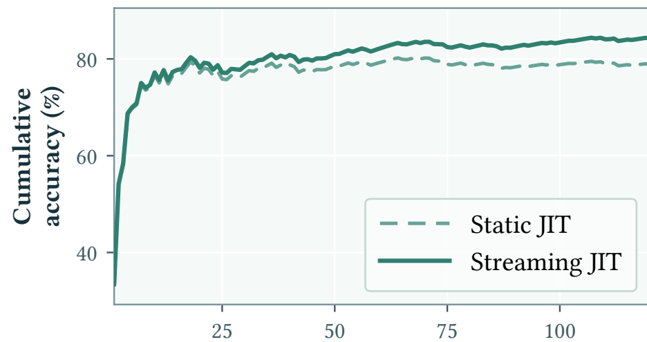
ShoppingPlanning
