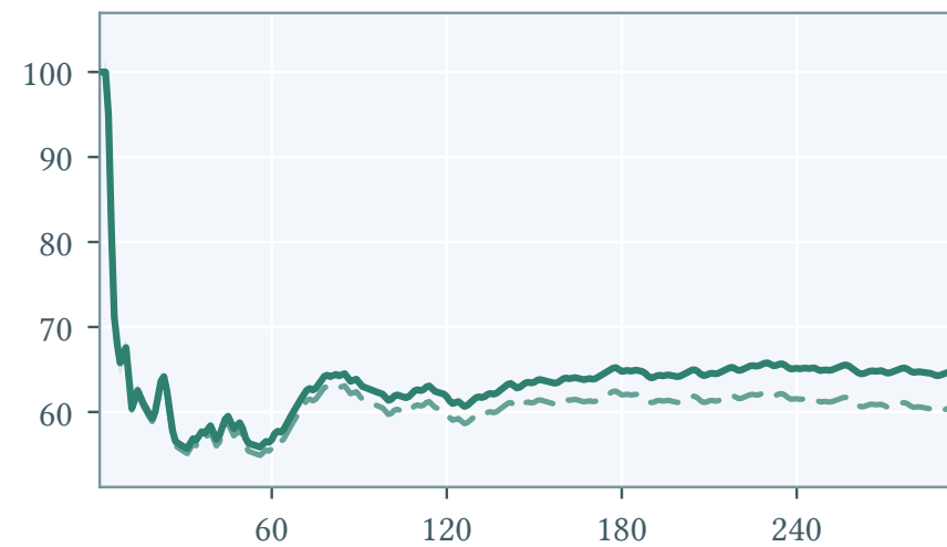
OfficeBench
