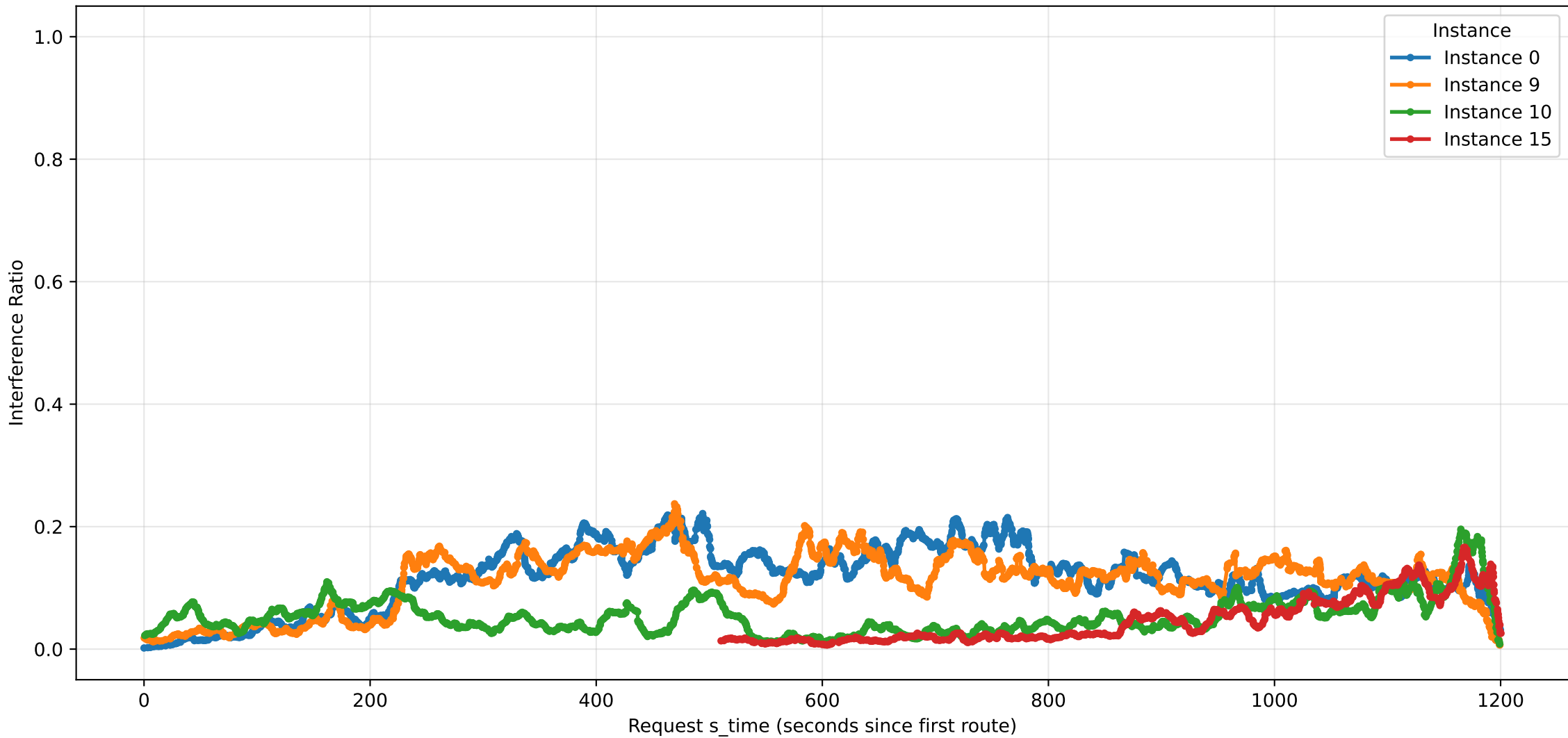
Per-Instance Decode Interference Ratio (Least-Ptks)
