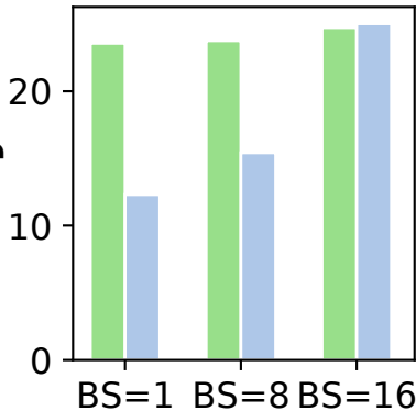
Chameleon-7B
