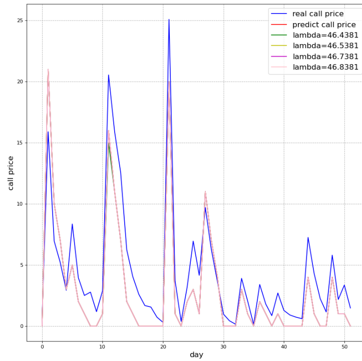
Figure 10: Sensitivity in terms of \lambda
