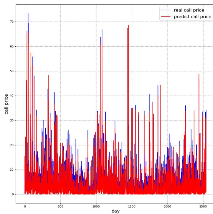
Figure 5: Black-Scholes-Merton for any time to maturity in MKS
