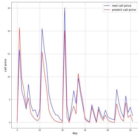
(b) Black-Scholes-Merton equation in predicting call prices in MKS when \tau = 31
