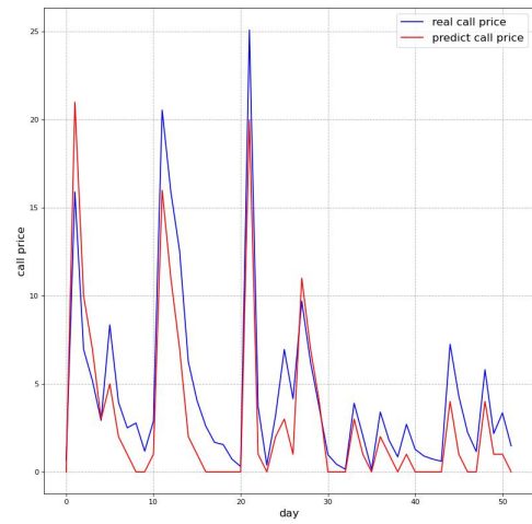
(b) Merton's jump diffusion model in predicting call prices in MKS when \tau = 31
