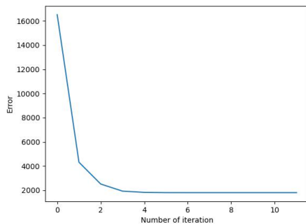
(a) Convergent rate of Black-Scholes-Merton equation
