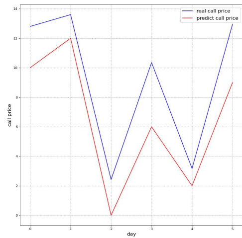
(d) Merton's jump diffusion model in predicting call prices in MKS when \tau = 183
