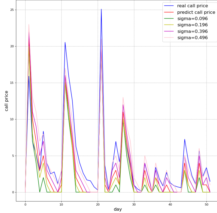
Figure 13: Sensitivity in terms of \sigma
