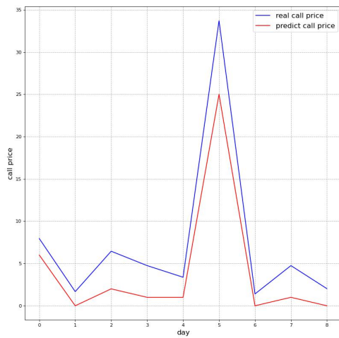
(c) Merton's jump diffusion model in predicting call prices in MKS when \tau = 92
