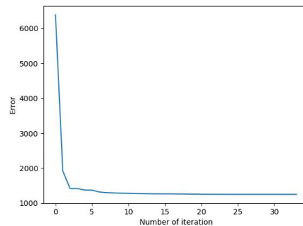
(b) Convergent rate of Merton jump diffusion
