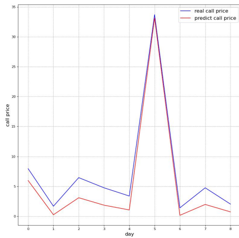
(c) Black-Scholes-Merton equation in predicting call prices in MKS when \tau = 92
