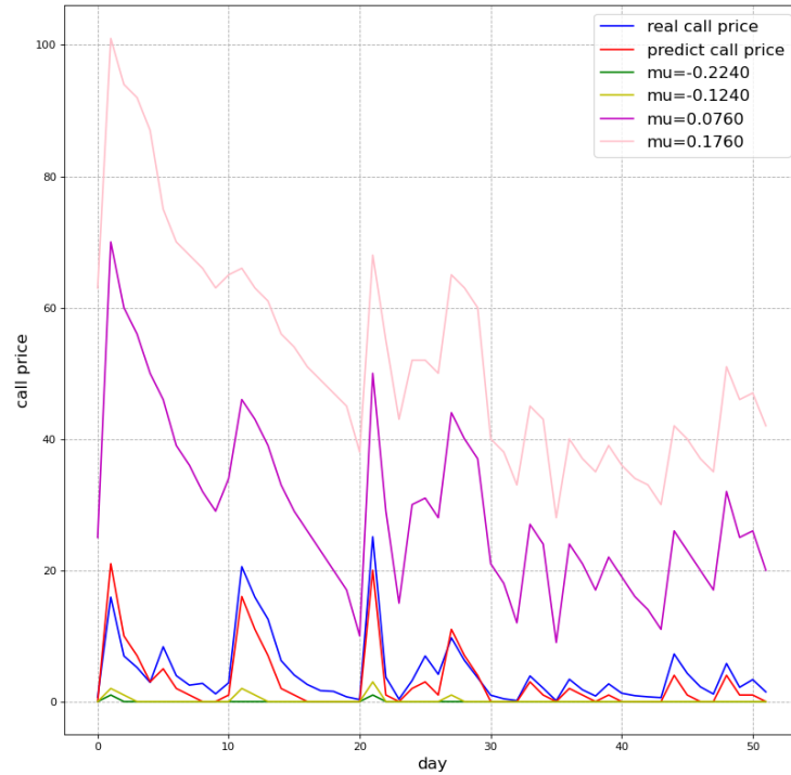
Figure 11: Sensitivity in terms of \mu
