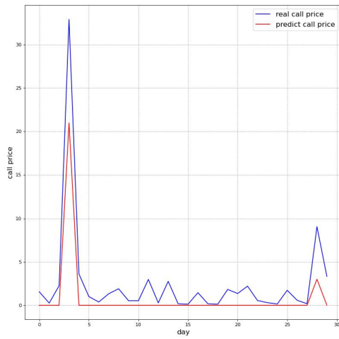
(a) Merton's jump diffusion model in predicting call prices in MKS when \tau = 1
