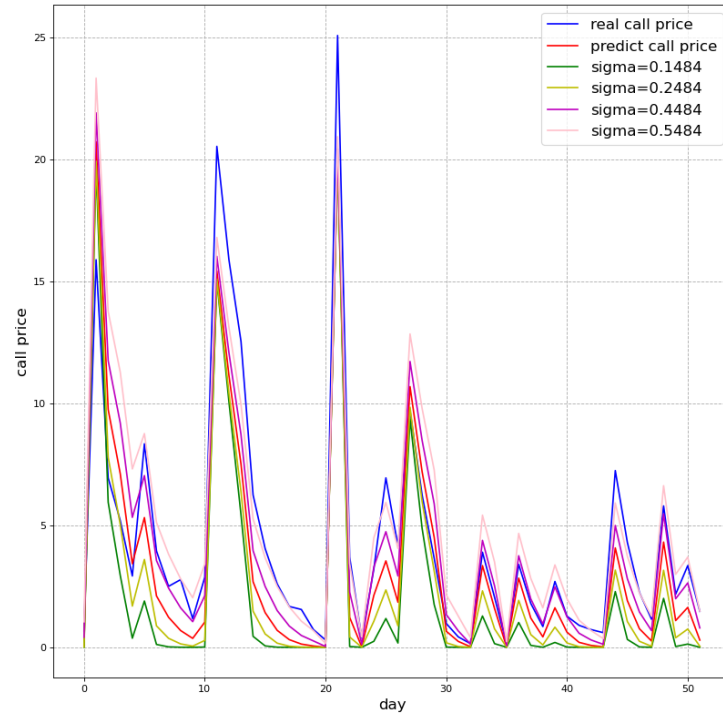
Figure 8: Sensitivity in Black-Scholes-Merton equation
