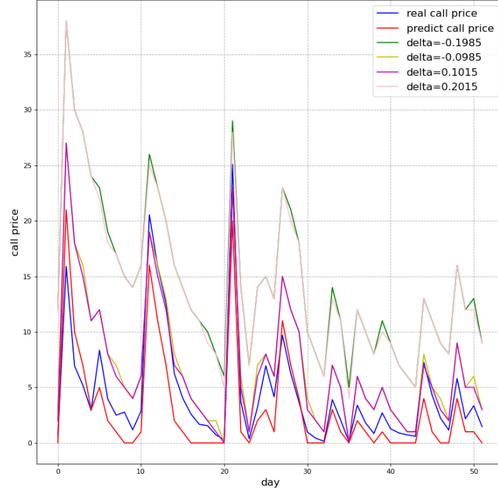
Figure 12: Sensitivity in terms of \delta
