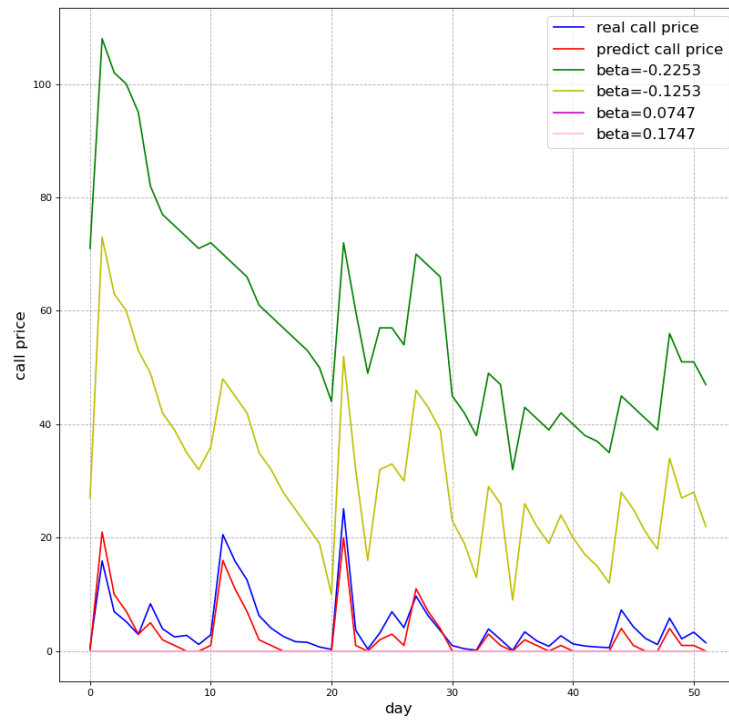
Figure 9: Sensitivity in terms of \beta
