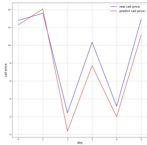
(d) Black-Scholes-Merton equation in predicting call prices in MKS when \tau = 183
