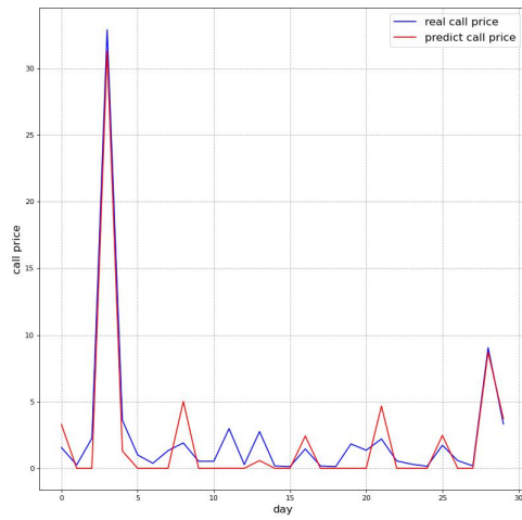
(a) Black-Scholes-Merton equation in predicting call prices in MKS when \tau = 1
