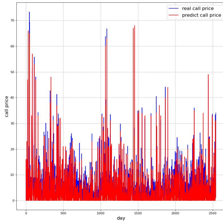
Figure 7: Merton's jump diffusion model for any time to maturity in MKS
