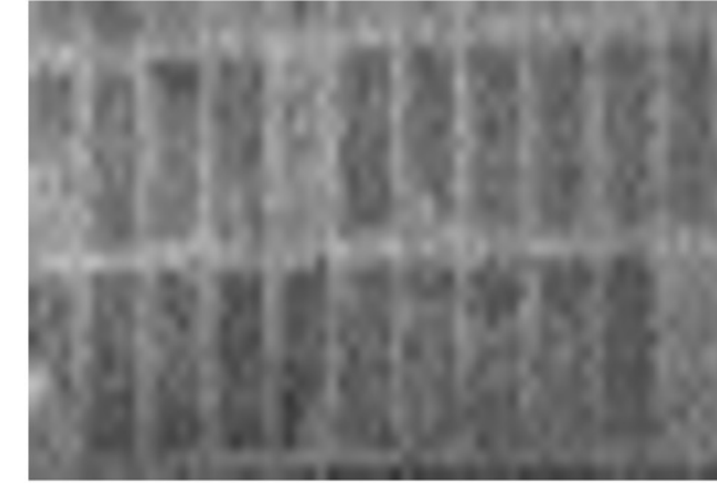
Noise
