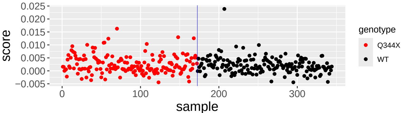
Rank = 3
