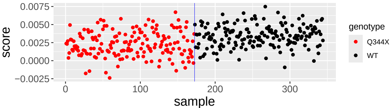
Rank = 3
