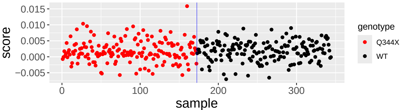
Rank = 2
