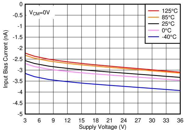
图 7-15. Input Bias Current vs. Supply Voltage
