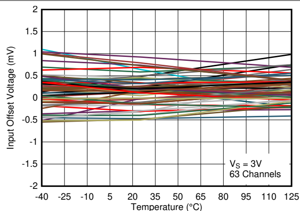
图 7-7. Input Offset Voltage vs. Temperature at 3V
