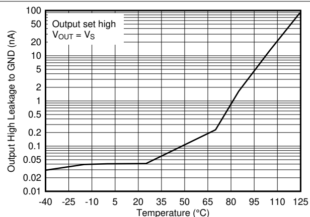
图 7-23. Output High Leakage Current vs. Temperature at 5V
