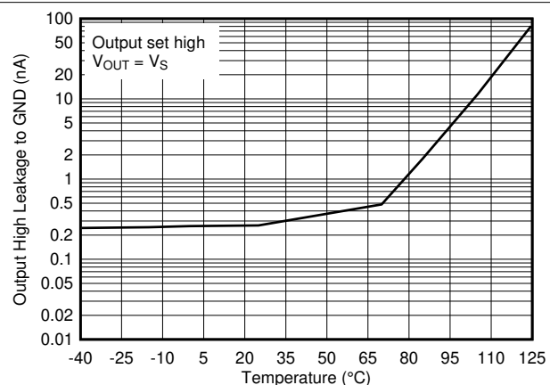
图 7-24. Output High Leakage Current vs. Temperature at 36V
