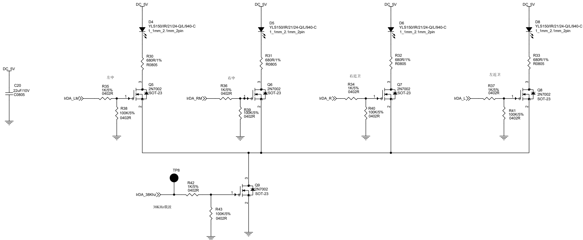
IR_LED 永林的IR_LED, 串阻680R 每个灯7.3mA
