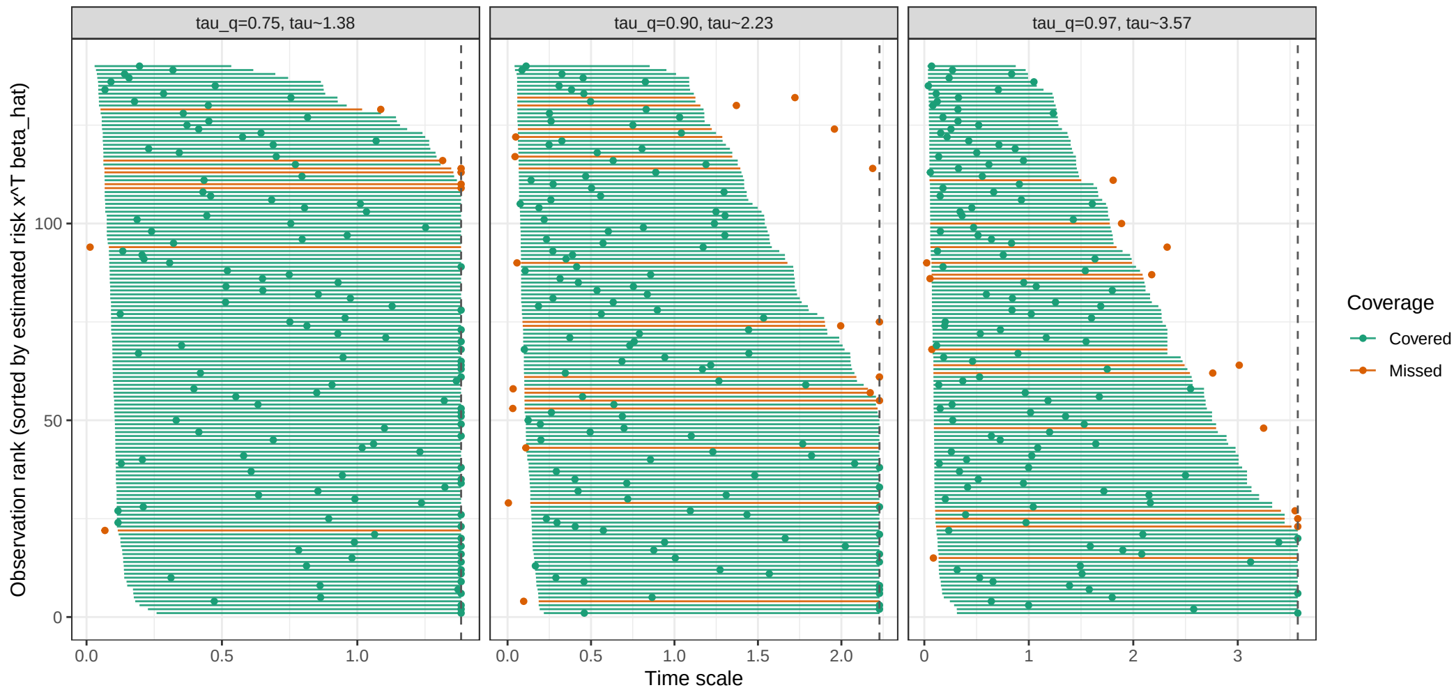
Sample-Level Intervals and Coverage by tau Setting
