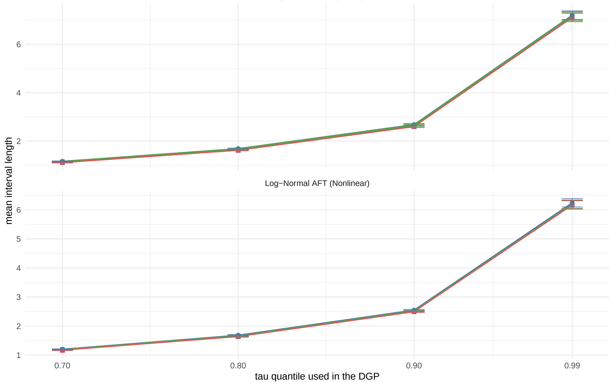
Log-Normal AFT (Linear)
