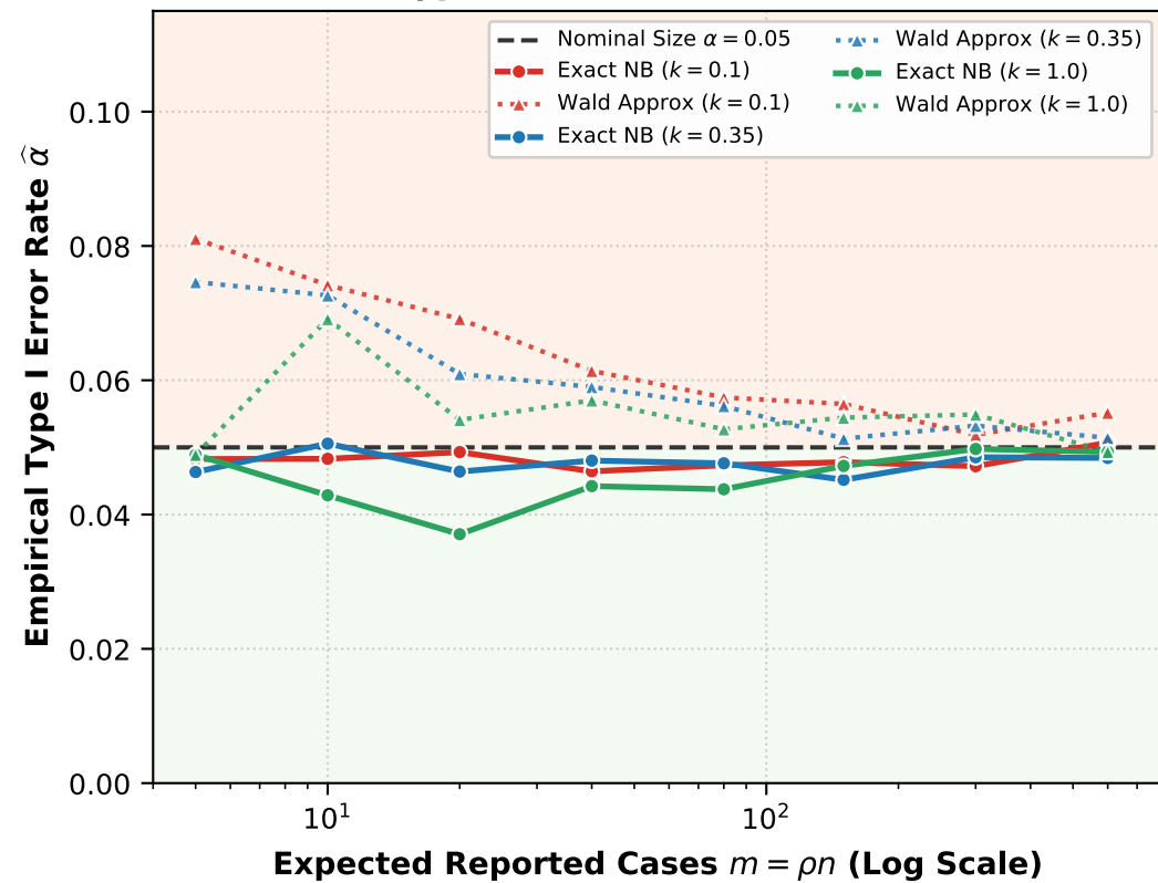
(a) Type I Error: Exact NB vs. Wald
