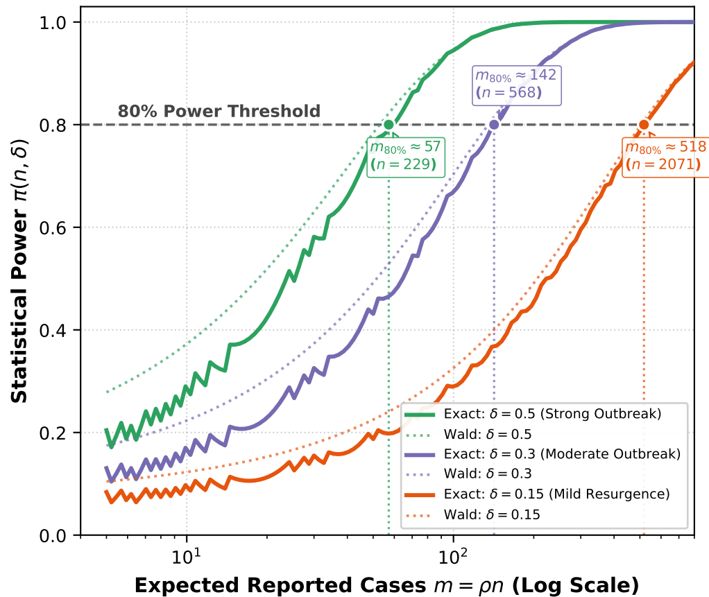
(b) Detection Power vs. Scale ( k = 0.35, \rho = 0.25 )
