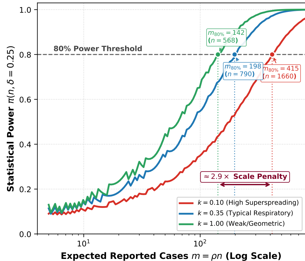
(c) Impact of Superspreading k on Surveillance Capacity
