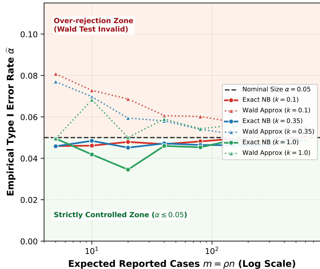
(a) Type I Error Control: Exact vs. Wald
