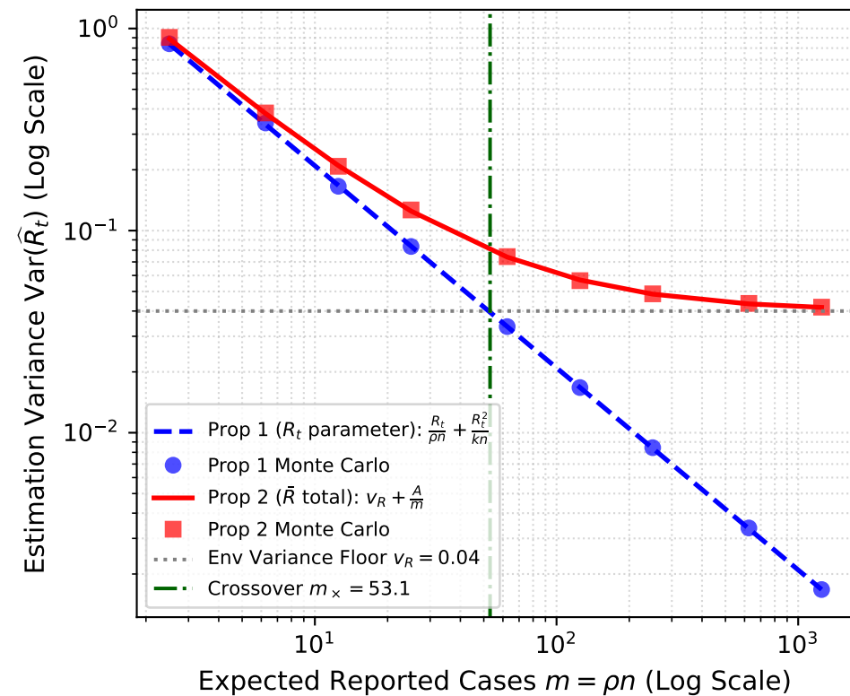
(a) Variance Convergence & Floor v_R
