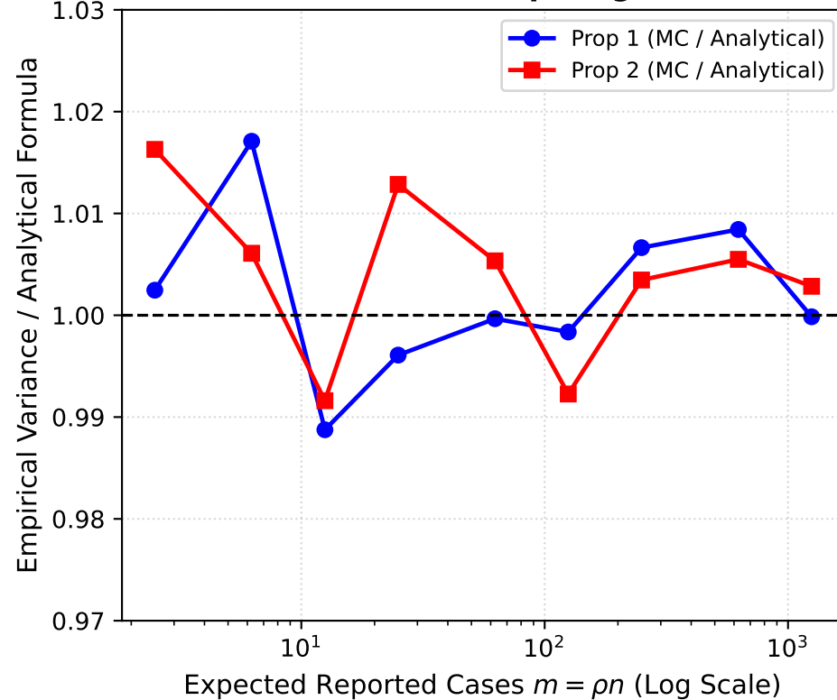
(b) Exact Finite-Sample Agreement
