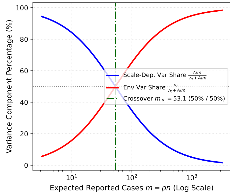
(c) Error Budget Transition Across m times
