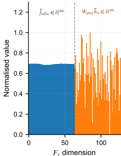
(c) Final 128-d F_v for transmission
