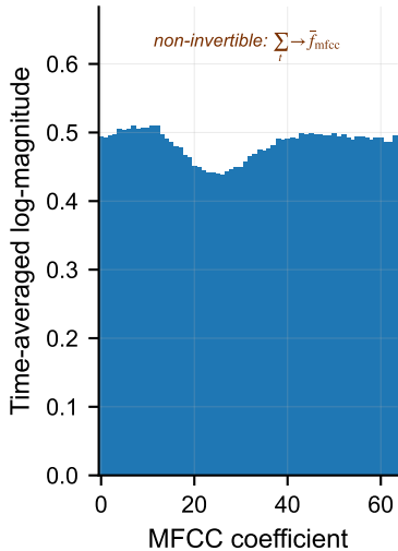
(b) Time-averaged 64-d MFCC
