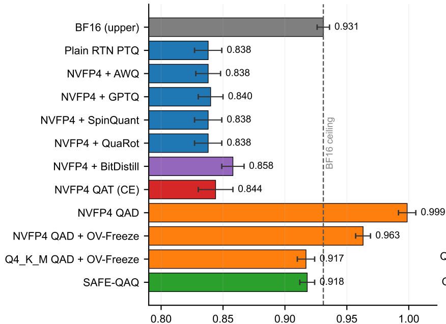
(a) F_1 across all methods
