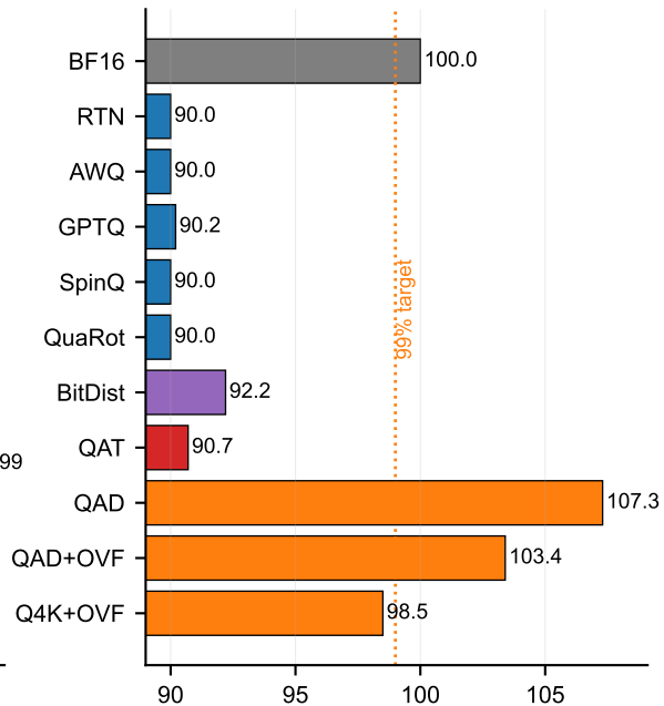
(b) Accuracy recovery
