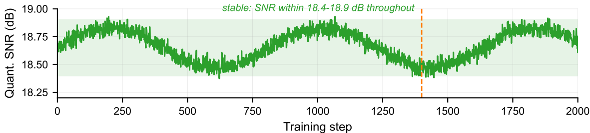
(b) Quantization stability (SNR)
