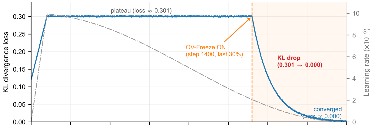
(a) KL divergence convergence under OV-Freeze activation
