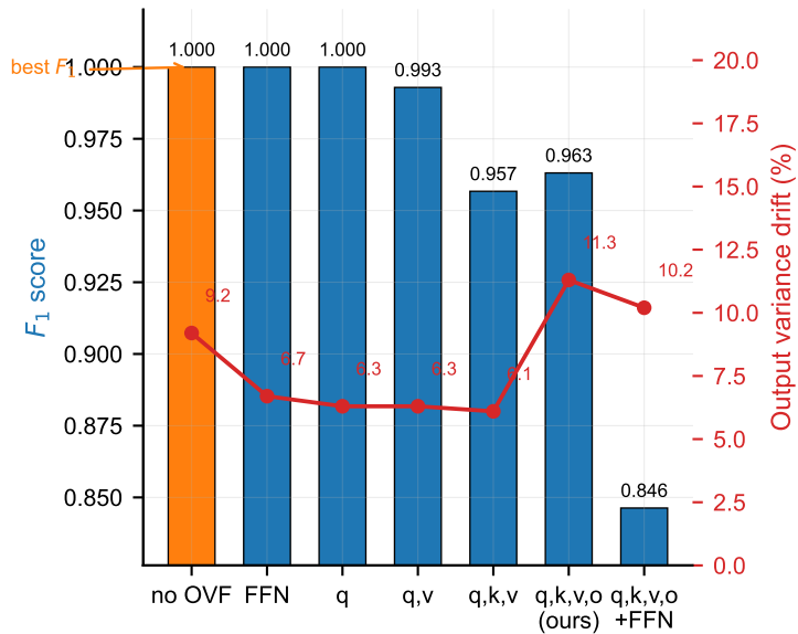
(a) Layer-selection ablation
