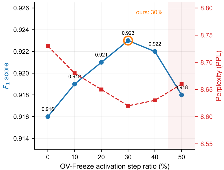
(b) Step-ratio ablation
