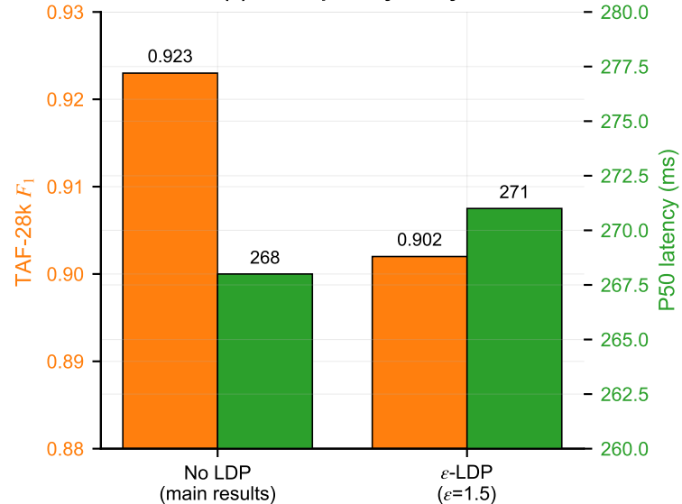
(c) \epsilon -LDP privacy-utility
