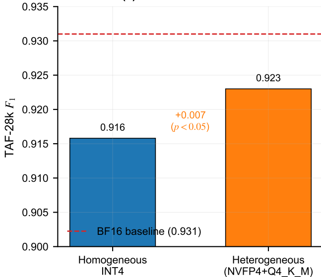
(a) Quantization scheme
