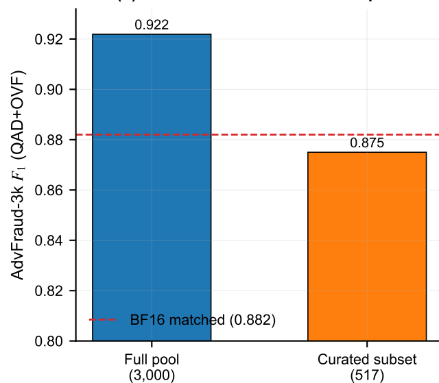
(b) AdvFraud-3k: curated vs full pool
