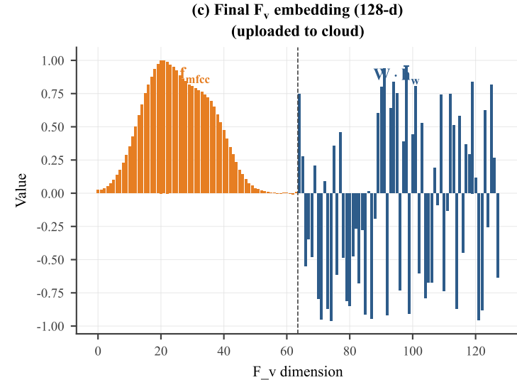
Fig. 10. Construction of the 128-d non-invertible acoustic embedding \mathbf{F}_{\mathbf{v}} . (a) Raw mel spectrogram contains full temporal information. (b) Time-averaging destroys phoneme order. (c) The final \mathbf{F}_{\mathbf{v}} concatenates MFCC and Whisper-projected features.
