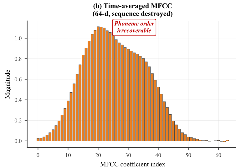
Fig. 10. Construction of the 128-d non-invertible acoustic embedding \mathbf{F}_{\mathbf{v}} . (a) Raw mel spectrogram contains full temporal information. (b) Time-averaging destroys phoneme order. (c) The final \mathbf{F}_{\mathbf{v}} concatenates MFCC and Whisper-projected features.
