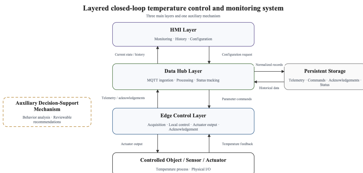
Figure 3.1 – General architecture of the developed system
